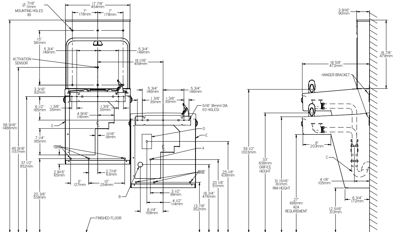
REDUCE HEIGHT BY 3" FOR INSTALLATION OF CHILDRENS ADA COOLER
