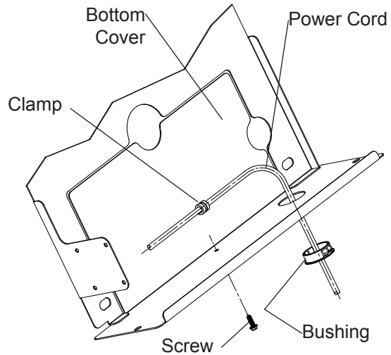
220V Power Cord Detail
